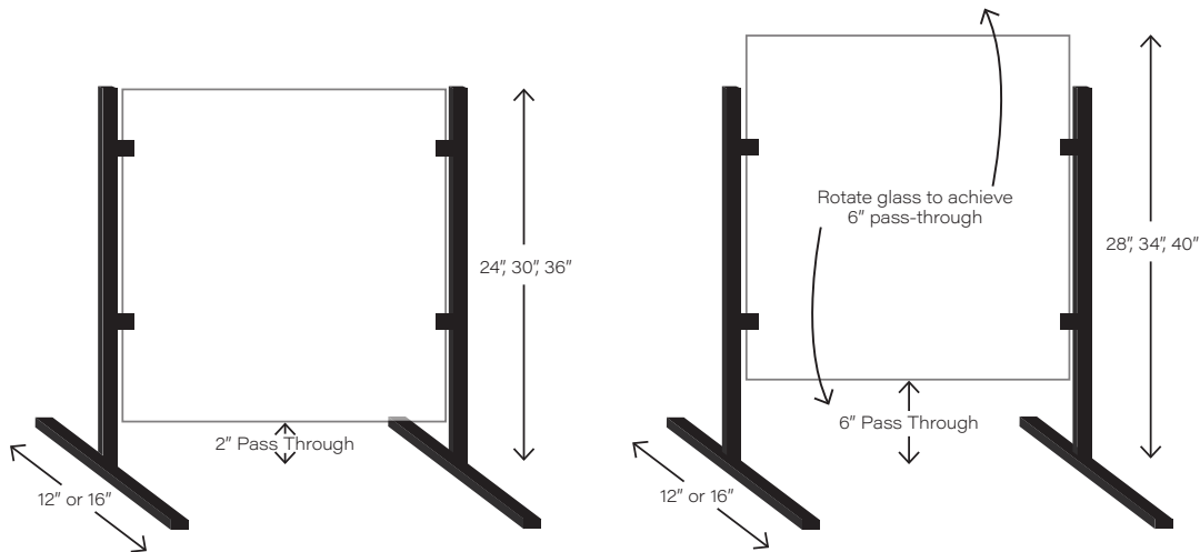
Clamps fasten through glass to prevent separation or slippage.
